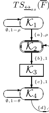
FIG. 4. The quotient transition system of \bar{F} for F = [(\{a\}, \rho) * ((\{b\}, \mathfrak{h}_k^1); (((\{c\}, \mathfrak{h}_l^0); (\{d\}, \theta)_1) \square ((\{c\}, \mathfrak{h}_m^0); (\{d\}, \theta)_2))) * \text{Stop}]
