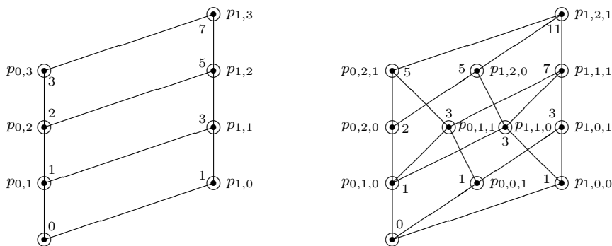
FIGURE 5. Hasse diagrams for T_{3,=}^P and T_{3,<}^P
