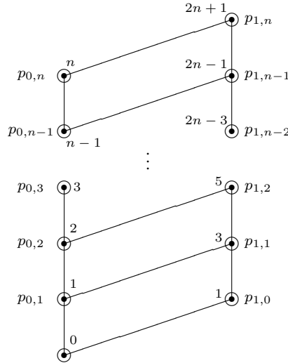
FIGURE 7. Hasse diagram for T_{n,=}^P
