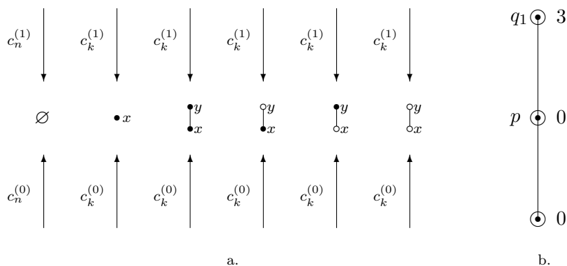
FIGURE 2. Realizations of p(x) (a.); and Hasse diagram of RK(T_1) (b.)
