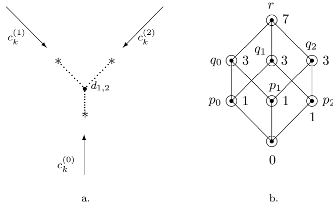
FIGURE 3. Here, d_{1,2} is the meet of strictly decreasing sequences of constants (c_k^{(1)})_{k \in \omega} and (c_k^{(2)})_{k \in \omega} , and the character * means one of the \{\emptyset, \bullet, \circ\} (a.); RK(T_2) is a Hasse diagram with boolean of \{p_0, p_1, p_2\} , here the type q_0 = p_0 \cup p_1 , q_1 = p_0 \cup p_2 , q_2 = p_1 \cup p_2 , r = p_0 \cup p_1 \cup p_2 (b.).
