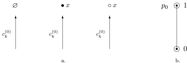
FIGURE 1. From left to right: a prime model, where there is no element greater than all c_k^{(0)} , a prime model, where among the elements of large c_k^{(0)} there is the smallest element, and a limit model where among the elements of large c_k^{(0)} there is no the smallest element (a.); \text{RK}(T_0) is a linear order of two elements. In Hasse diagrams, we draw the realization of prime models over a certain set of formulas using the character \bullet based on the Rudin-Keisler preorder \leq_{\text{RK}} on the models. The circled circle \odot above the \bullet means the possibility of realization of limit models over these sets of formulas. It should be noted here that the total number of characters \bullet is the total number of prime models, and the numbers next to \odot mean the number of limit models (b.).
