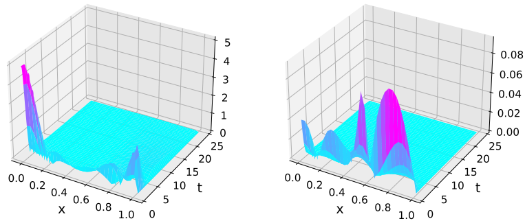
(a) |u_{l,j}^{\alpha,(2)} - u_{l,j}^{\alpha}|
